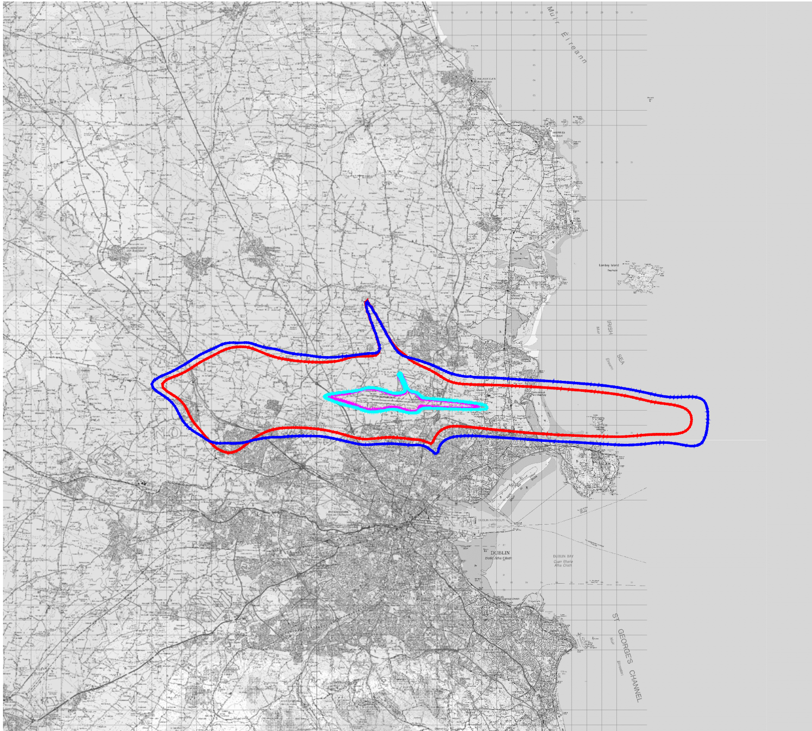
Figure 06 Comparison of 2020 and 2021 Annual L_{night} Noise Contours
